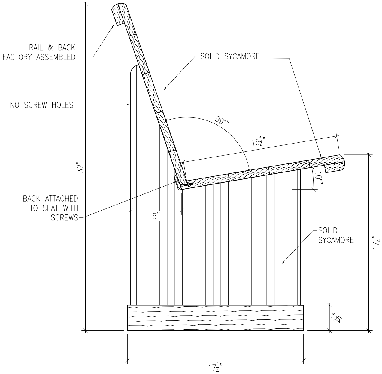
2 A VERTICAL SECTION MODEL "A" SCALE: 2" = 1'-0"
